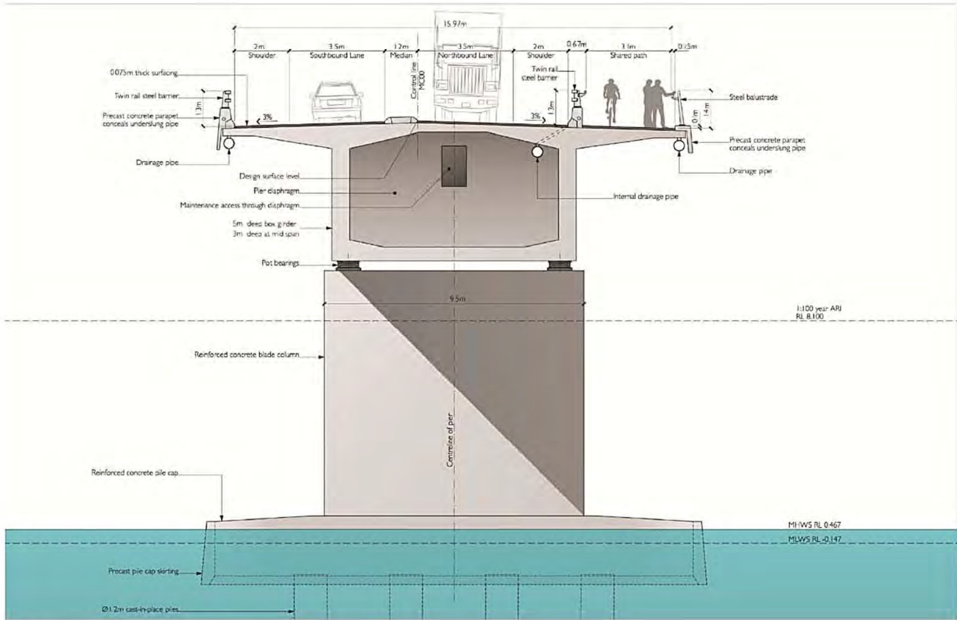
Bridge cross-section 2 (bridge spanning river)
