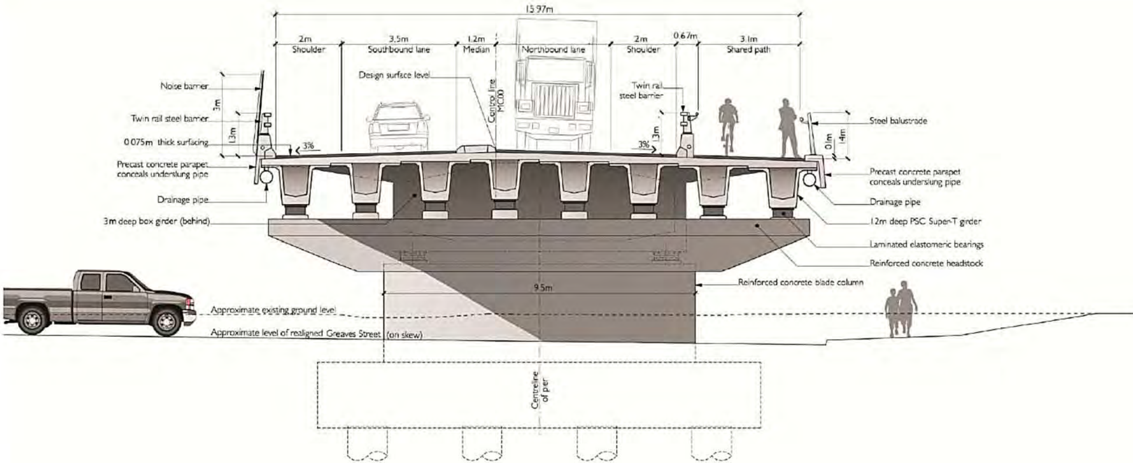
Bridge cross-section 3 (northern end of the bridge)
