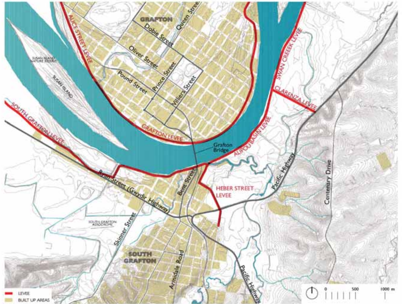
Figure 2.6: Grafton levee system
