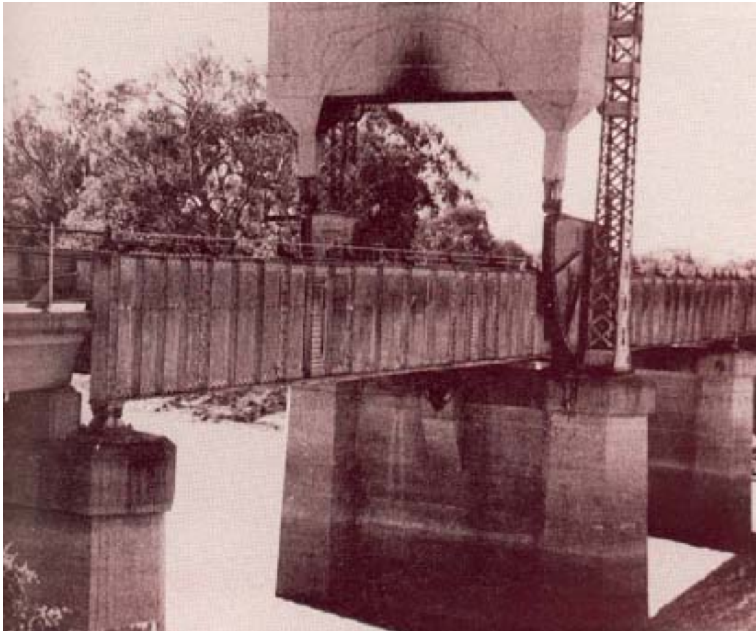
Figure 3: View of the Menindee Bridge in 1958 showing the concrete counterweight and the associated towers that have since been removed (DMR, 1977:7).
