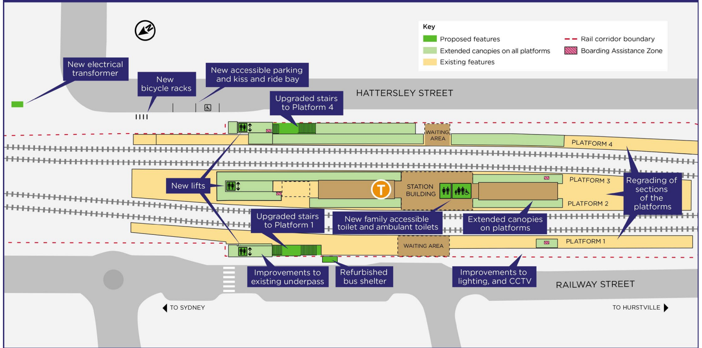
Indicative layout of Banksia Station Upgrade, subject to detailed design
